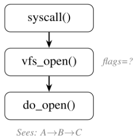
Figure 2: Edge coverage reports identical paths for different argument values. Data-flow extraction reveals the security-relevant difference.
