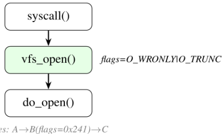
Figure 2: Edge coverage reports identical paths for different argument values. Data-flow extraction reveals the security-relevant difference.
